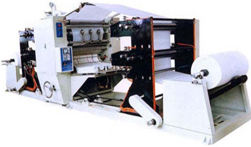
YX-CHMJ-200/2 Automatic Box-drawing Face Tissue Machine
