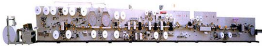
YX-HY-180D Three-folding Independent Packaging Winged Sanitary Napkin Production Line
